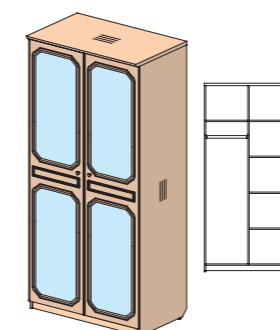
20H211 1000x600x2130
