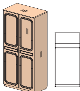
20H110 1000x600x2130
